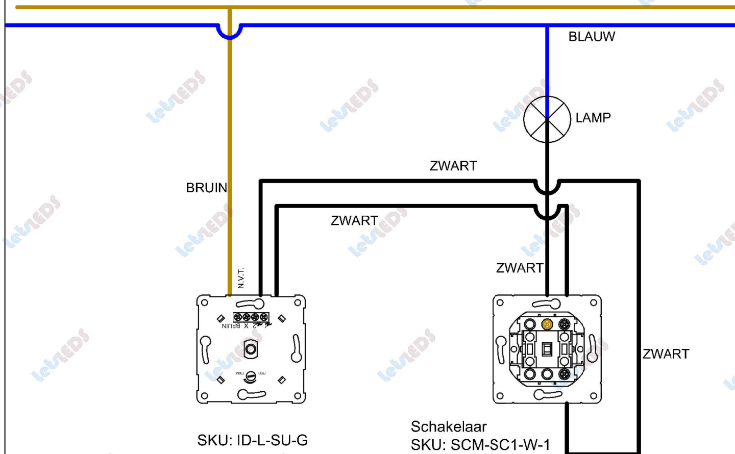
hotel schakeling
