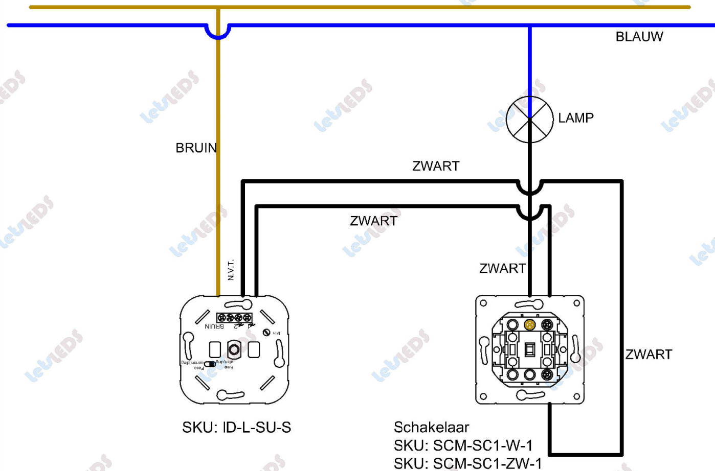
hotel schakeling
