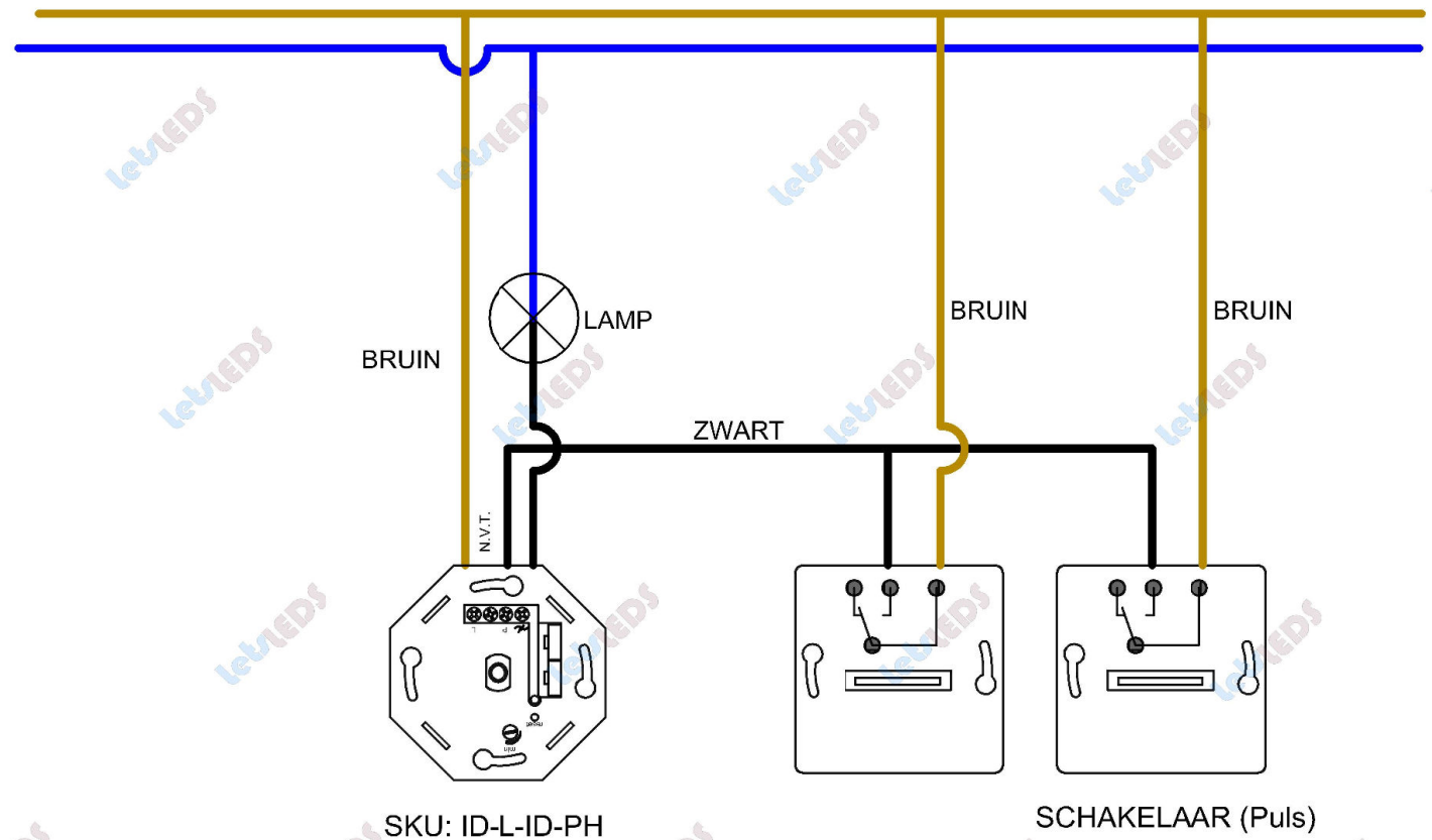
hotel schakeling
