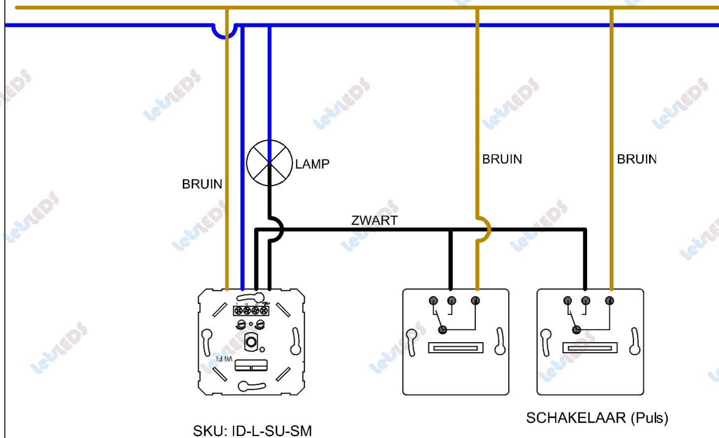
hotel schakeling
